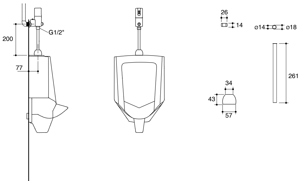
Product Diagram
