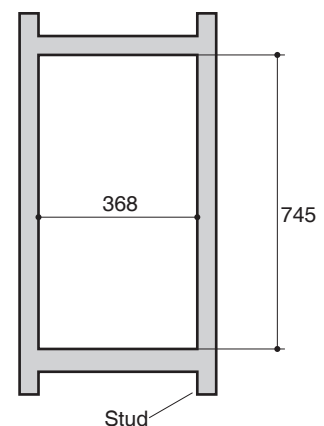
Rough-In for Recessed Installation
